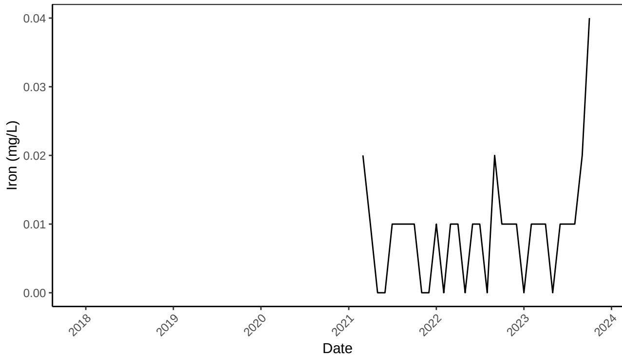
B2 Raceway 2 Iron (mg/L) Monthly Median
